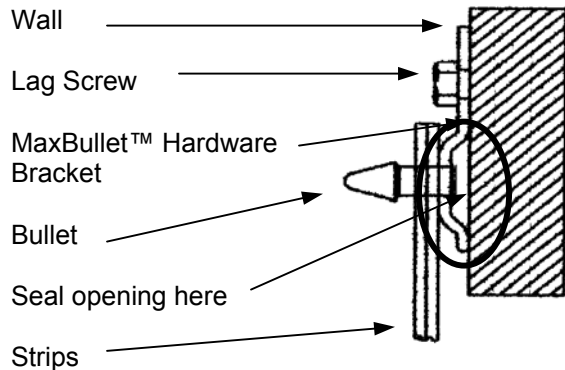
Diagram 1 Side View
