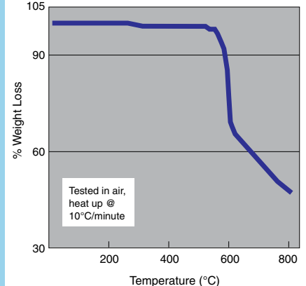
Thermogravimetric Analysis (TGA) Meldin® 7001
