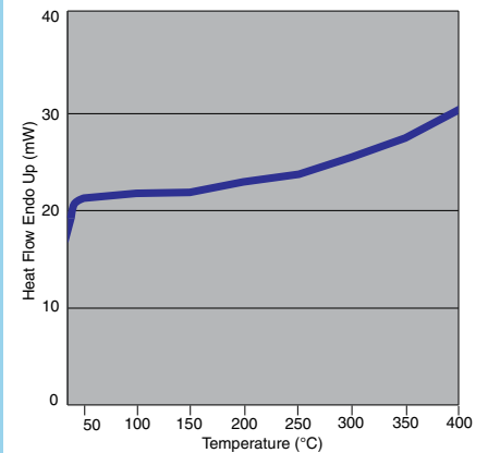
Differential Scanning Calorimetry (DSC) Meldin® 7000 Series
